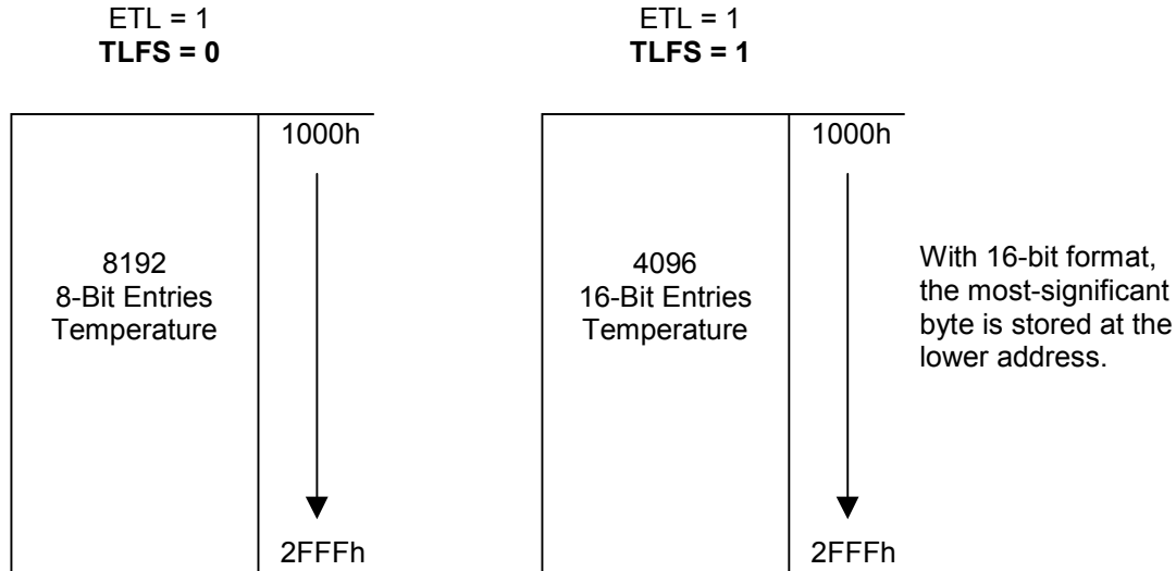
Figure 7. Temperature Logging
